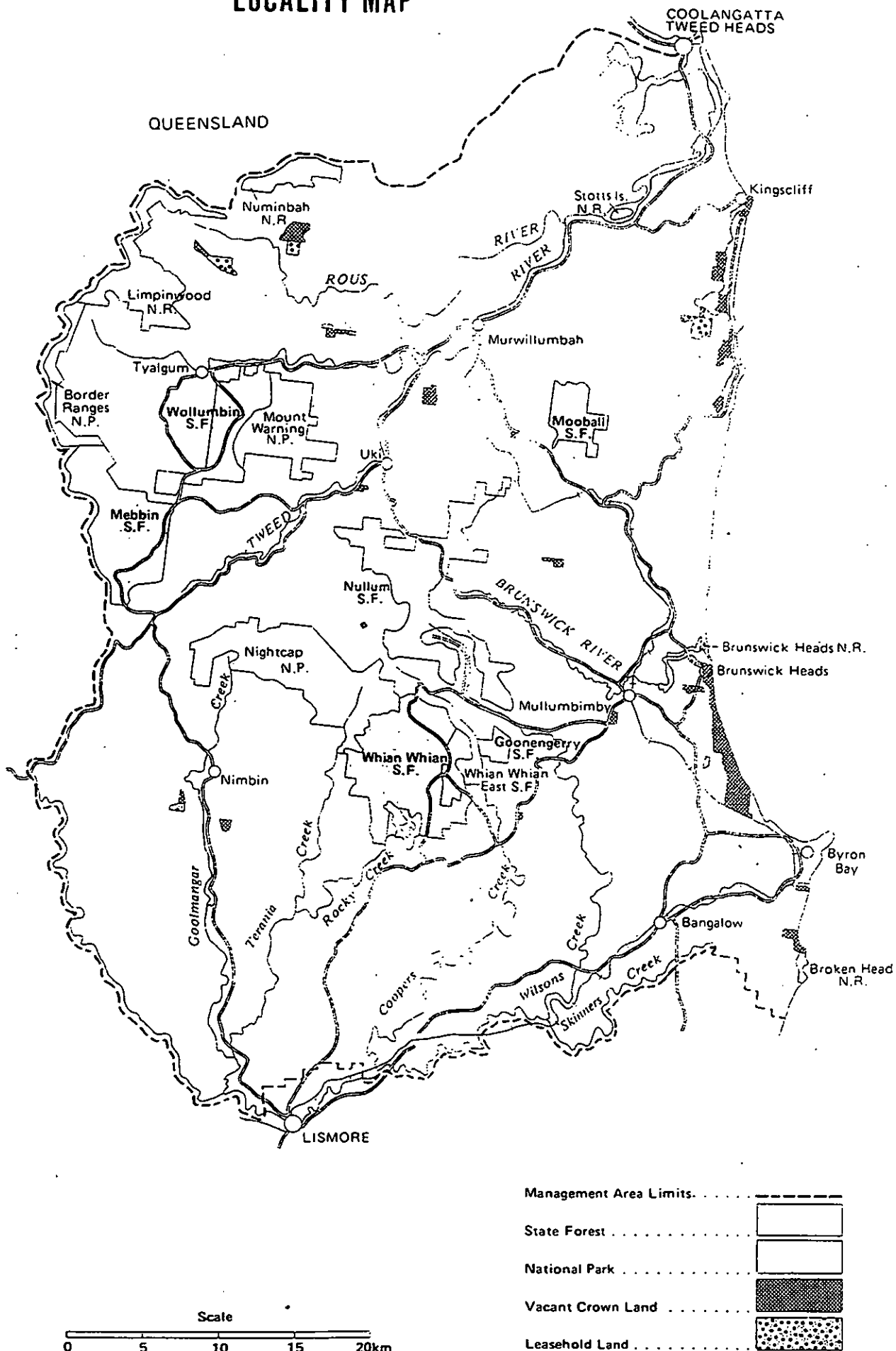
Figure 3. Location of the State Forests in the Murwillumbah Forest Management Area. (Reproduced from the Murwillumbah Forest Management Plan),
