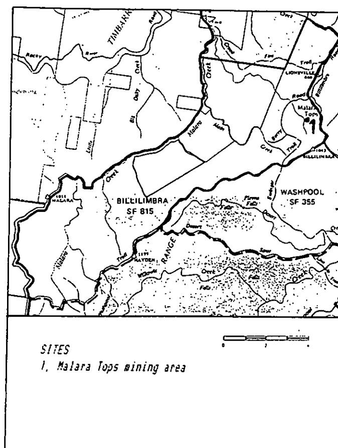
Figure 6. Sites in Billilimbra State Forest. (Produced from the Tenterfield State Forests 1:125 000 map)
